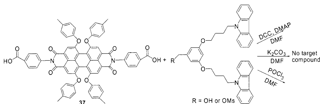
Scheme 6. Attempts to synthesize target imide-type dendrimers according to conventional synthetic ester protocols and tosylation.
