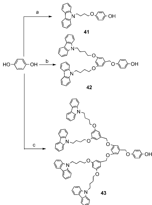
Scheme 9. Synthetic route to dendrons 41 , 42 , and 43 for the bay-type dendrimers. Reagents and conditions: a) N -(4-bromobutyl)-9 H -carbazole, K_2CO_3 , 18-crown-6, acetone, reflux, 36 h; b) 27 , K_2CO_3 , 18-crown-6, acetone, reflux, 60 h; c) 34 , K_2CO_3 , 18-crown-6, acetone, reflux, 60 h.
