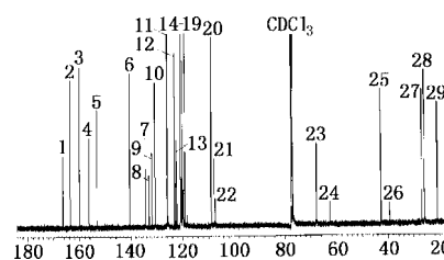
Figure 2. ^{13}C NMR spectrum of dendrimer 3 .
