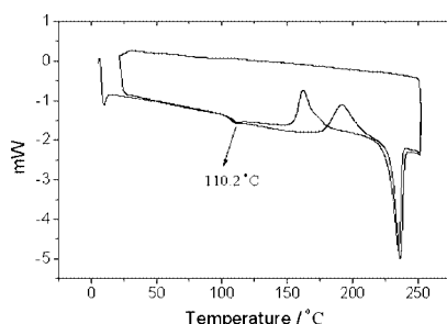
Figure 4. DSC trace of dendrimer 3 .
