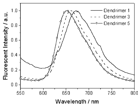
Figure 6. Normalized fluorescence spectra of dendrimers 1 , 3 , and 5 in solid film excited at 460 nm.
