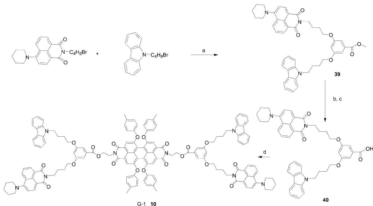
Scheme 8. Synthetic route to target dendrimer 10 . Reagents and conditions: a) methyl 3,5-dihydroxybenzoate, K_2CO_3 , 18-crown-6, THF, reflux, 60 h; b) KOH, THF/methanol, reflux, 20 h; c) 10% HCl; d) N,N' -bis(2-hydroxyethyl)-1,6,7,12-tetrakis(4-methylphenoxy)-3,4,9,10-perylenebis(dicarboximide), DCC, DMAP, CH 2 Cl 2 , room temp., 24 h.
