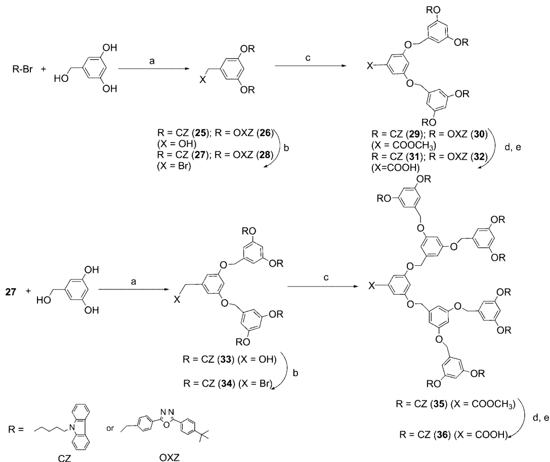
Scheme 5. Synthetic route to G-2 and G-3 dendrons of imide-type dendrimers. Reagents and conditions: a) K_2CO_3 , 18-crown-6, acetone, reflux, 60 h; b) CBBr_4/PPh_3 , CH_2Cl_2 ; c) methyl 3,5-dihydroxybenzoate, K_2CO_3 , 18-crown-6, THF, reflux, 60 h; d) KOH, THF/methanol, reflux; e) 10% HCl.
