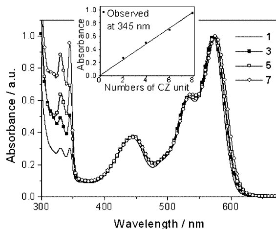
Figure 5. Normalized absorption spectra of dendrimers 1 , 3 , 5 , and 7 in THF ( 2.0 \times 10^{-5}\text{ M} ). Inset: Plot of number of carbazole units in dendrimer vs. absorbance at 345\text{ nm} .
