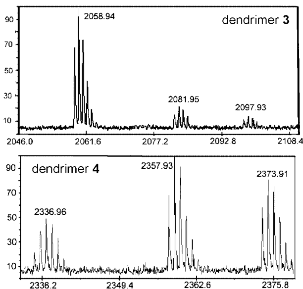
Figure 3. MALDI-TOF mass spectra of dendrimers 3 (top) and 4 (bottom).
