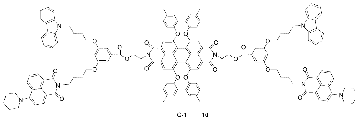
Scheme 2. Chemical structure of cascade energy-transfer imide-type dendrimers.
