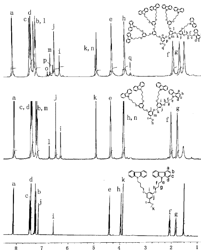
Figure 1. ^1H NMR spectra of dendrons 17 (G-1), 29 (G-2), and 35 (G-3).
