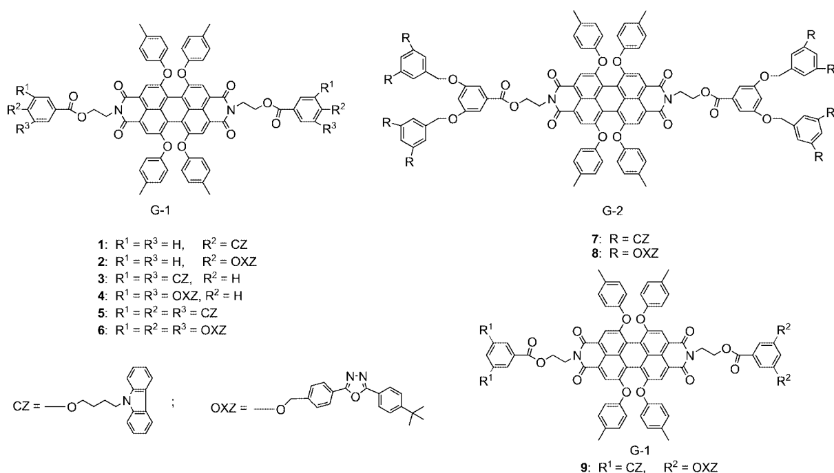
Scheme 1. Chemical structures of CZ- or OXZ-terminated imide-type dendrimers.
