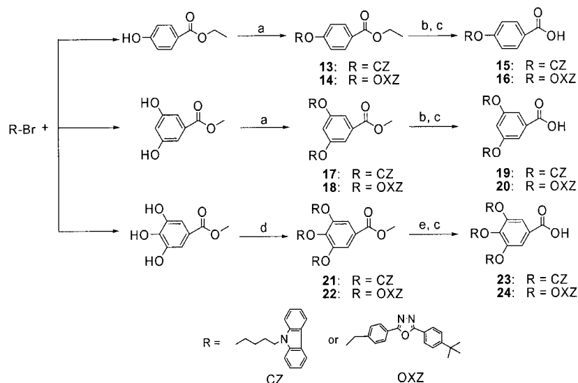
Scheme 4. Synthetic route to G-1 dendrons of imide-type dendrimers. Reagents and conditions: a) K_2CO_3 , 18-crown-6, acetone, reflux, 60 h; b) KOH, THF/methanol, reflux, 10 h; c) 10% HCl; d) K_2CO_3 , 18-crown-6, THF, reflux, 60 h; e) KOH, THF/methanol, reflux, 16 h.
