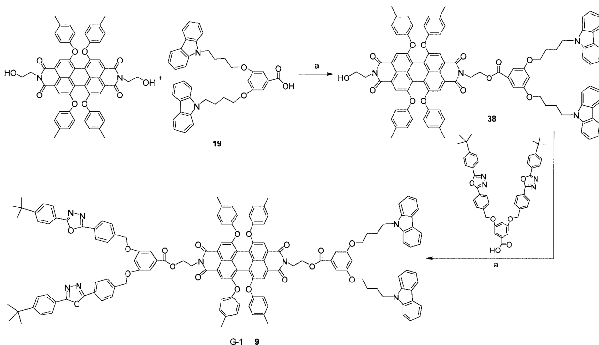
Scheme 7. Synthetic route to target dendrimer 9 . Reagents and conditions: a) DCC, DMAP, \text{CH}_2\text{Cl}_2 , room temp., 24 h.
